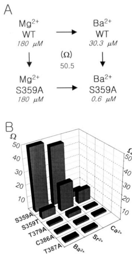
FIGURE 8 Mutant cycle analysis between amino acid residues lining the conduction pore and intracellular divalents. (A) Representative mutant cycle showing the interaction between a residue in the P-region, Ser-359, and a divalent cation, Ba^{2+} . The current blockade by intracellular Mg^{2+} and Ba^{2+} were measured for wild-type (WT) and S359A mutant channels in a pair-wise manner, and the inhibition constant ( K_i ) were shown in italics. A coupling coefficient, \Omega , was calculated using an equation, \Omega = \{K_i(\text{WT}, Mg^{2+}) \times K_i(\text{S359A}, Ba^{2+})\} / \{K_i(\text{WT}, Ba^{2+}) \times K_i(\text{S359A}, Mg^{2+})\} . When Ser residue was replaced for Ala at the position and the intracellular Mg^{2+} was substituted for Ba^{2+} , a strong energetic coupling, \Omega = 50.5 , was observed. (B) \Omega map of amino acid residues in rSK2 channel and intracellular alkali earth metals. The inhibition constants ( K_i ) of three divalent cations ( Ca^{2+} , Sr^{2+} , and Ba^{2+} ) on mutant channels of four different positions were obtained in pair-wise manners. \Omega of each channel:ion pair was calculated from four K_i values in the mutant cycle, and plotted as bars in the graph. The K_i value of Mg^{2+} on wild-type channel, 180 \mu\text{M} , was used arbitrarily as the control. \Omega of T387: Ca^{2+} was not determined.
