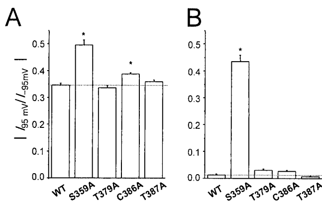
FIGURE 5 Bar graphs represent the degree of current rectifications in wild-type and mutant channels in the presence of 2 \mu\text{M} intracellular \text{Ca}^{2+} (A) and 2 \mu\text{M} intracellular \text{Ca}^{2+} and 10 \mu\text{M} \text{Ba}^{2+} (B). The ionic currents measured at 95 mV were divided into the currents at -95 mV and the absolute values ( |I_{95\text{mV}}/I_{-95\text{mV}}| ) were plotted for each channel (*, p < 0.001 ).
